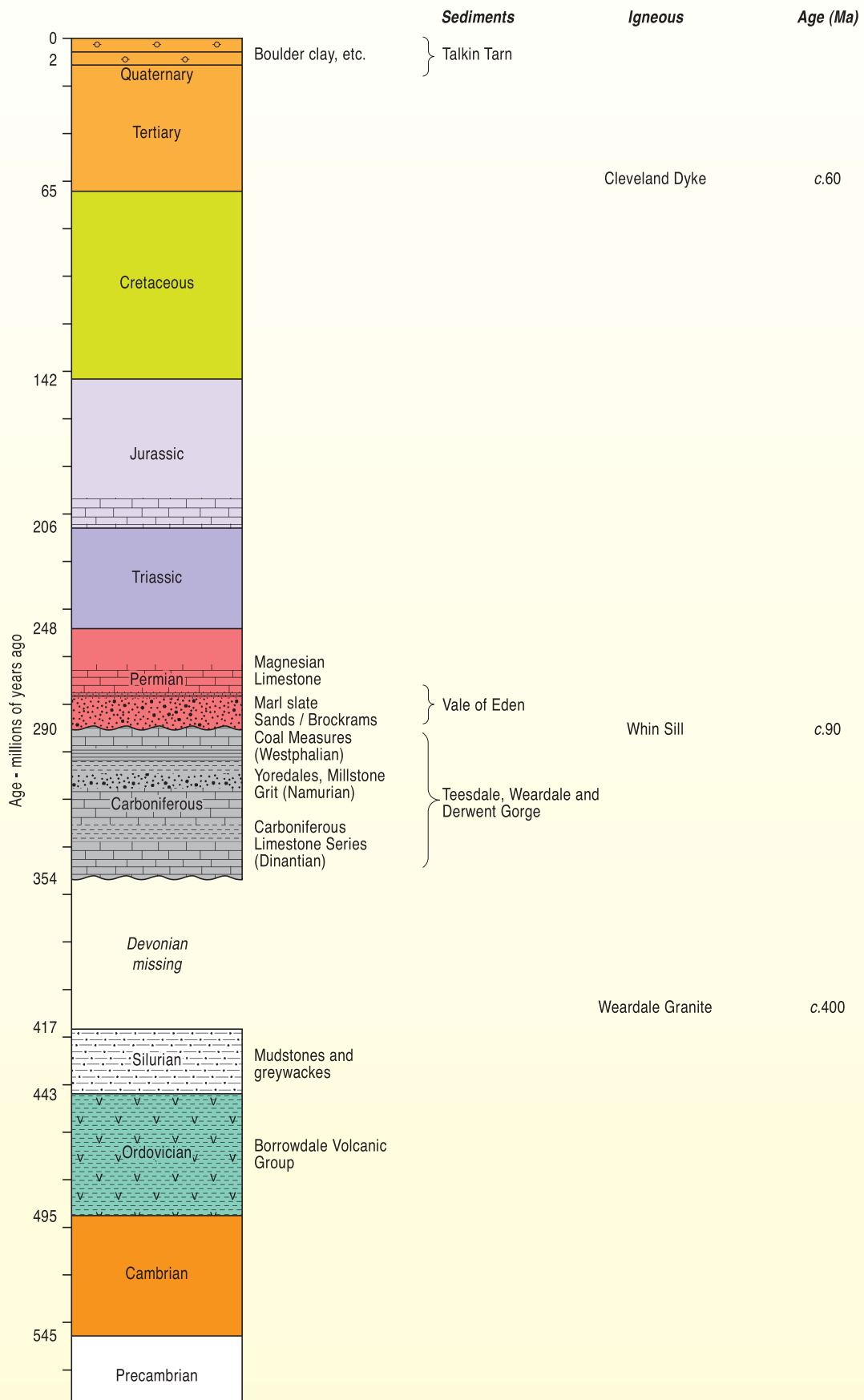
Figure 1: Geological time
